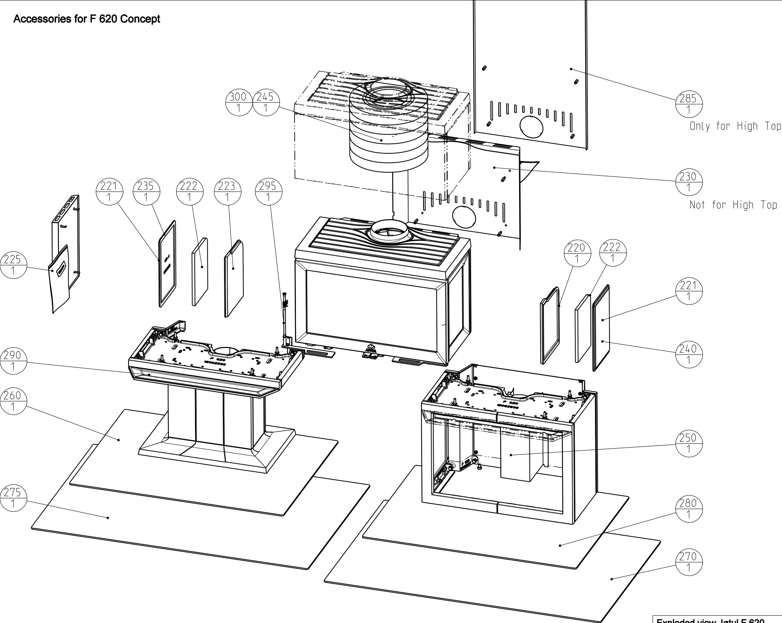
Exploded view Jøtul F 620
